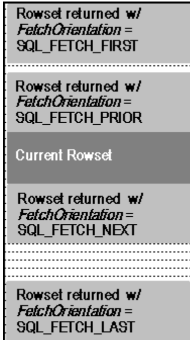
Figure 11.4 Fetching next, prior, first, and last rowsets
