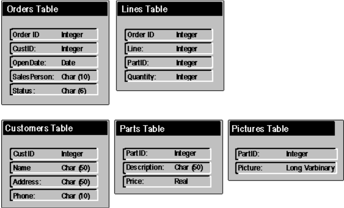
Figure 7.1 Sales order database structure
